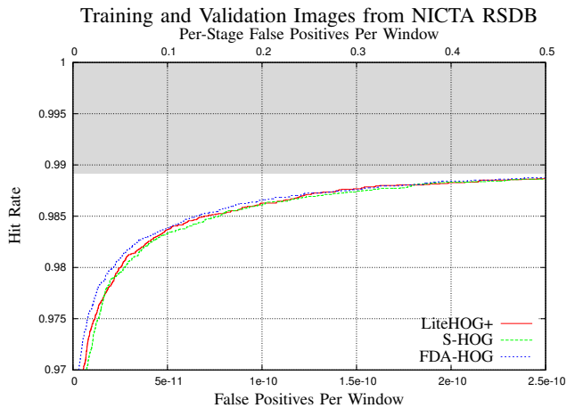
Fig. 4. Fifth stage ROC performance using training and validation images obtained using the NICTA Road Scene DataBase. Surprisingly the performance of each of the three features is almost equivalent. Upon closer inspection of the classifiers we found that the S-HOG and FDA-HOG features achieved much higher detection rates than LiteHOG+ on training data. This suggested that the S-HOG and FDA-HOG features were overfitting patterns in the training data more severely. See Section VI-A. The gray shaded area at the top of the plot indicates the accumulated false negative rate incurred by the previous four stages (see Table II).
